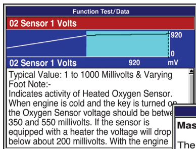
Typical Sensor/Data Values with live data Graphing.
